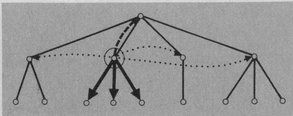
Figure 3. Tree traversals in Telidon. From the circled node, relative access is provided to the immediate ancestor (dashed line), immediate descendants (bold lines), and sibling pages (dotted lines) without reference to page identifiers.
