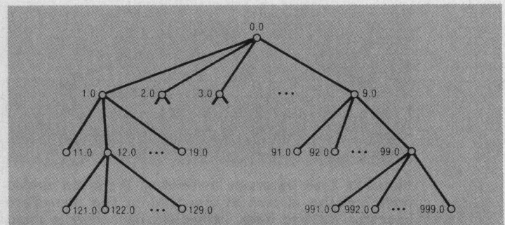
Figure 2. A tree of page nodes, using Telidon identifiers.
