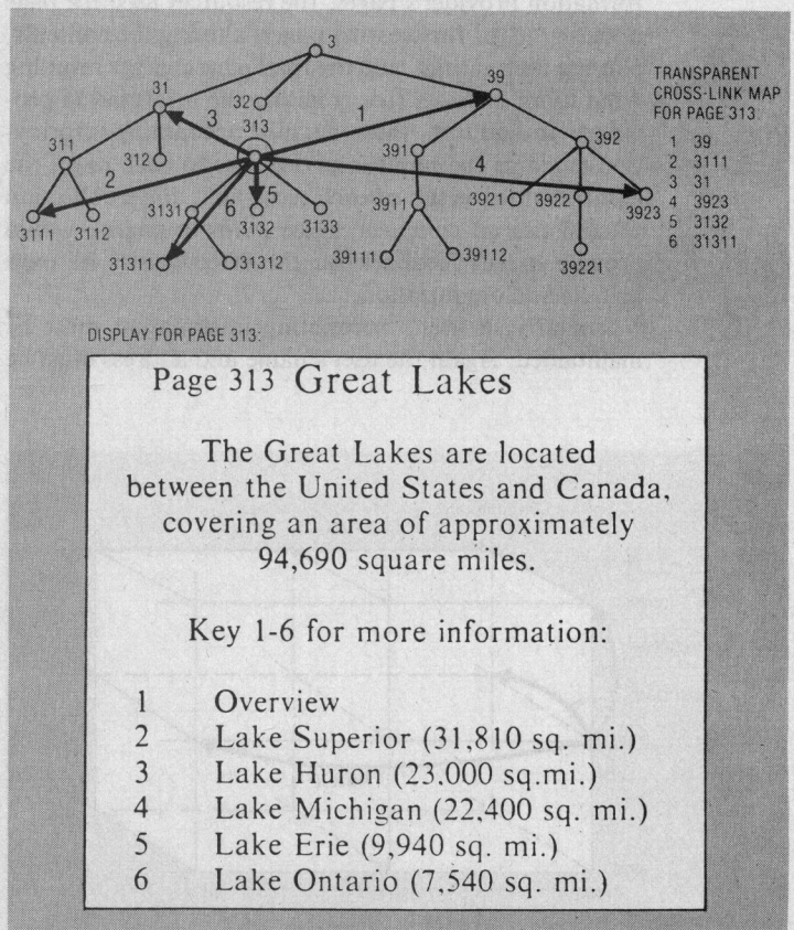
Figure 4. Cross-link map for user-oriented access structures.
